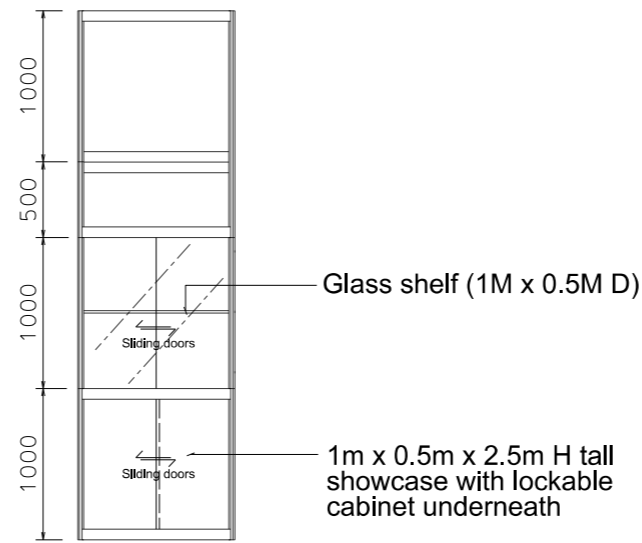
VIEW A
